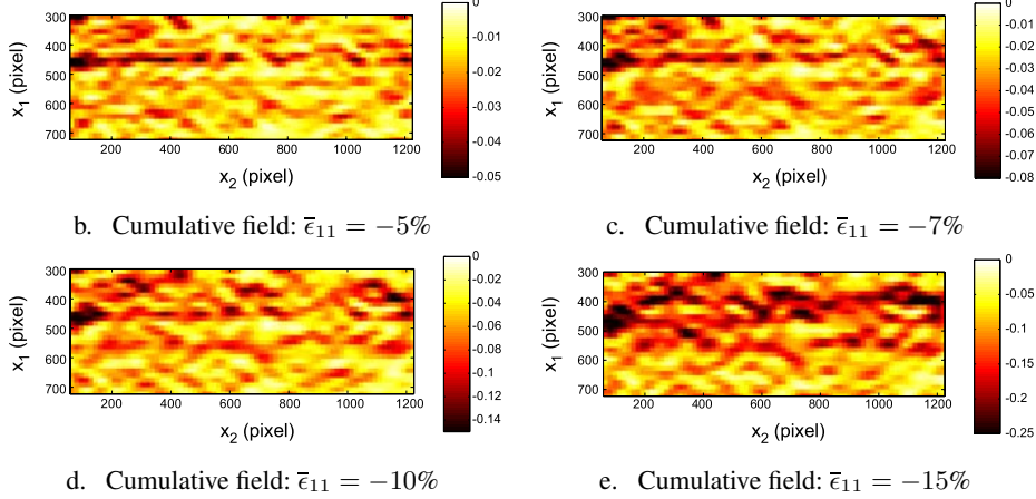
Figure 9. Initial texture orientation and cumulative \epsilon_{11} -field for different levels of the global strain. Correlation parameters: size of ZOI = 16 \times 16 pixels, \delta = 16 pixels. Scale: 1 pixel \Leftrightarrow 0.15 mm.
